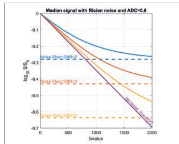
Figure 2: Logarithm of the median of 106 diffusion signal curves generated with ADC=0.8 \times 10^{-3} \text{ mm}^2/\text{s} , between b=0 and b=2000 , for different Rician noise SNR. The dashed lines indicate the noise floor. The purple solid line indicates the theoretical signal expected in the absence of noise.
